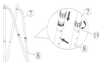
Figure 5. Angling Adjustment
